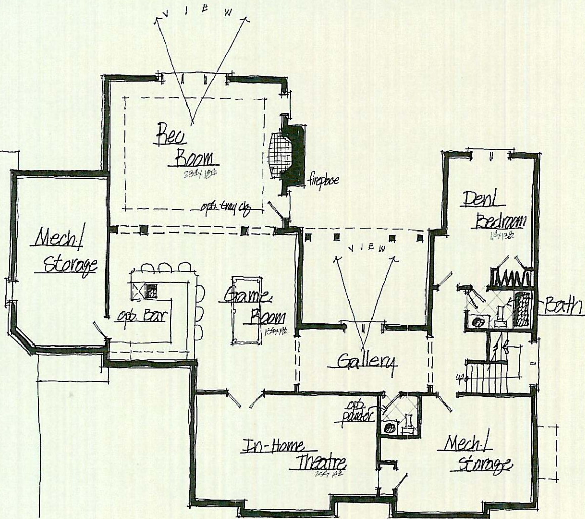
Lower Level Floor Plan The Stratford
